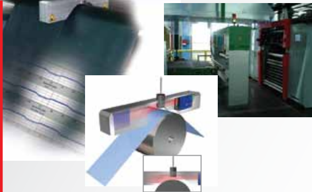
Innerliner thickness profile
